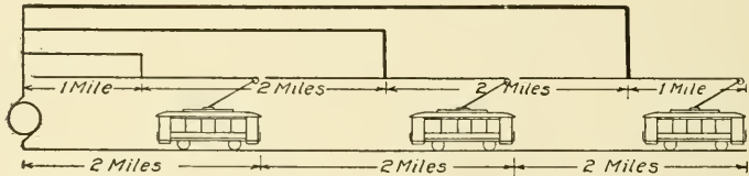
Fig. 209. Feeder System Using Separate Trolley Sections
